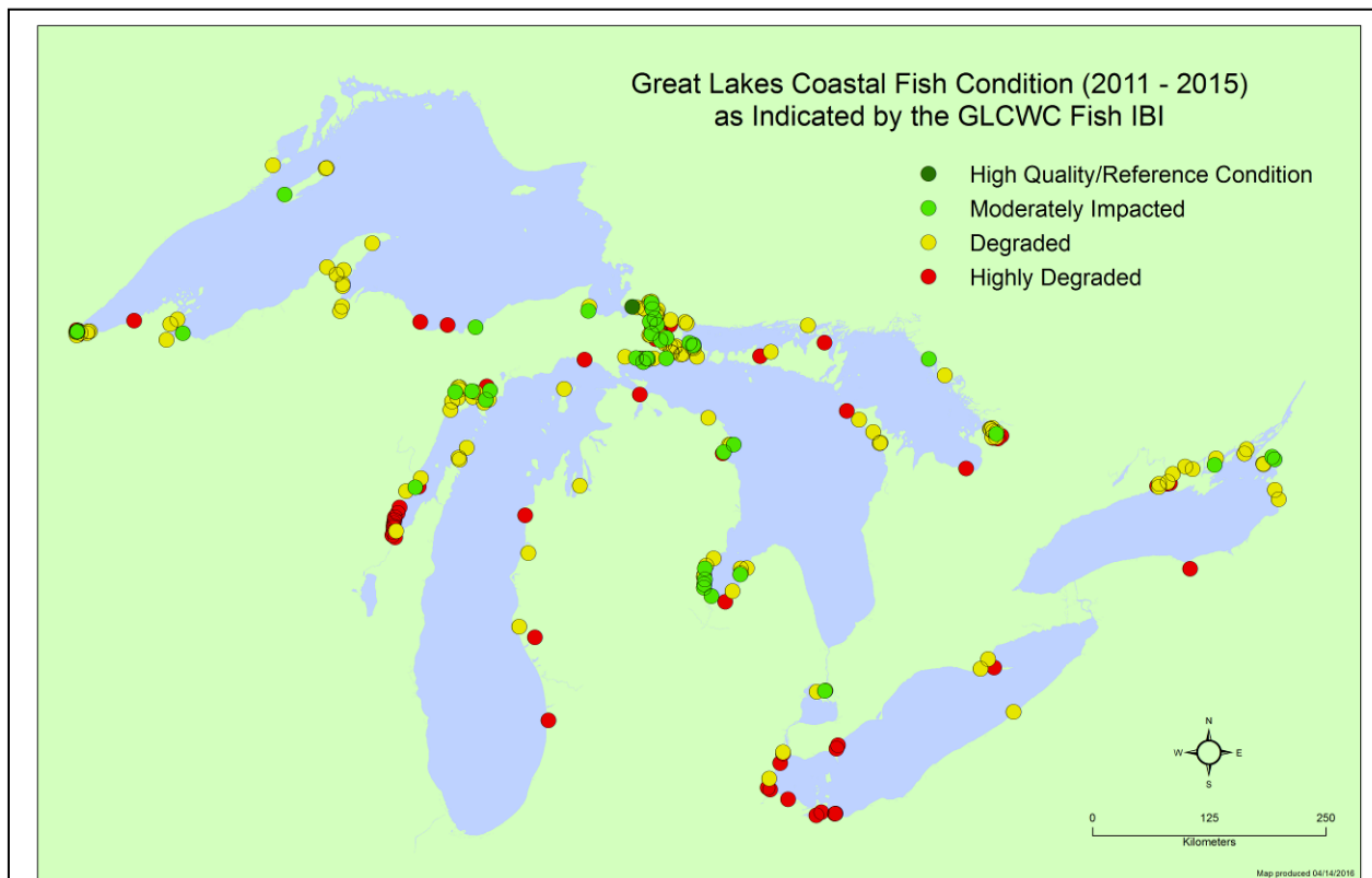
Figure 14. Condition of coastal wetland fish communities at sites with bulrush or cattail zones. The indicator is labeled “draft” while more zone IBIs are developed. Based on data from 2011 through 2015.
